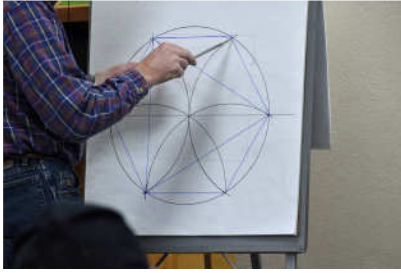
Straightedge and compass construction.
